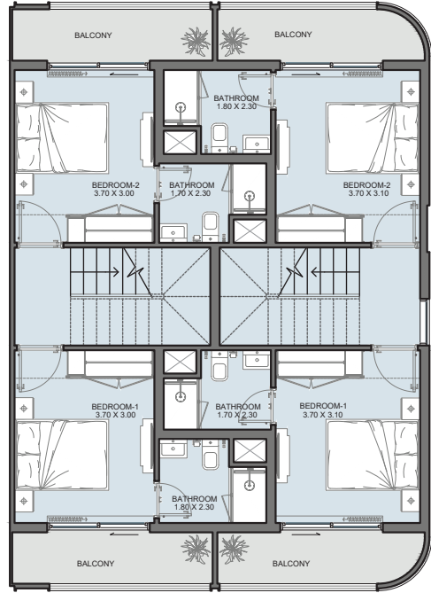
FIRST FLOOR Middle Unit FIRST FLOOR Corner Unit
