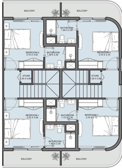
SECOND FLOOR Middle Unit SECOND FLOOR Corner Unit
