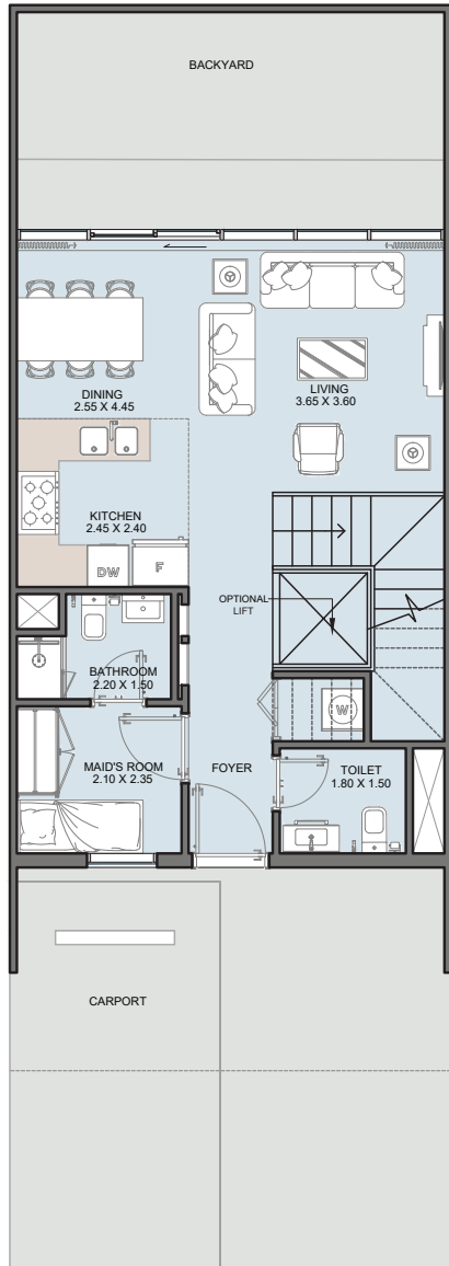
GROUND FLOOR Middle Unit
